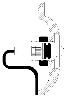
Installed, section view Custom water-tight mounting sleeve
